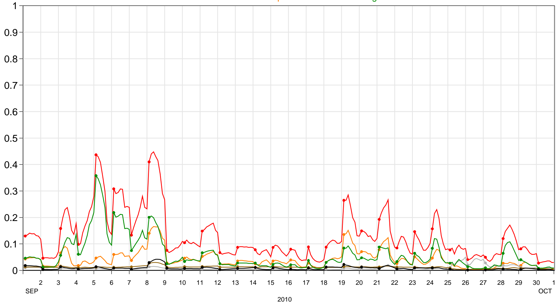
Comparison of model (f93i) and MODIS AOT at 550nm and L1.5 Aeronet AOT at 500nm over Yellowknife (62.45° N, 114.41° W). Model: 00UT, 1-30 Sep 2010, T+3 to T+24.
