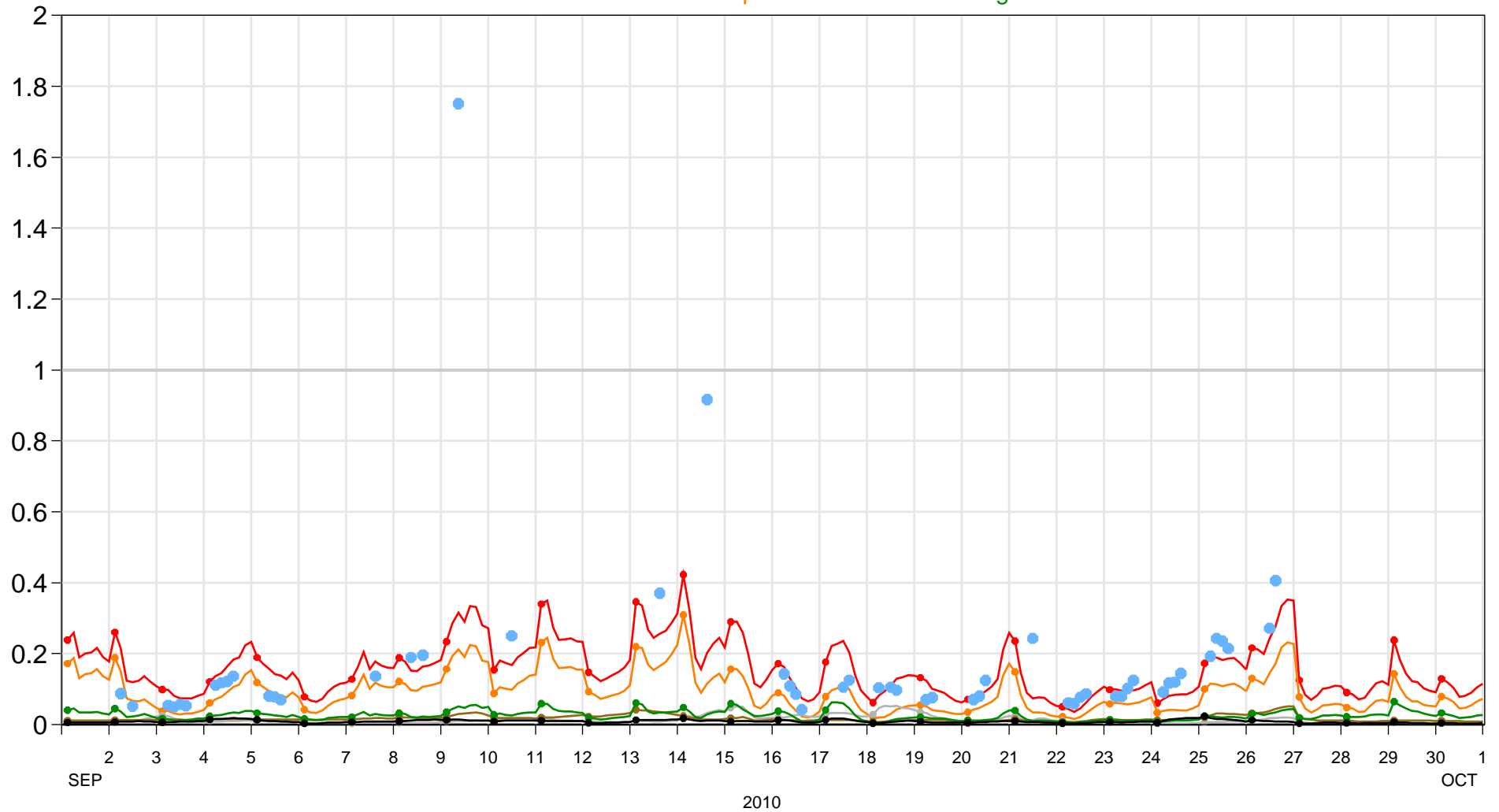
Comparison of model (f93i) and MODIS AOT at 550nm and L1.5 Aeronet AOT at 500nm over Belsk (51.84° N, 20.79° E). Model: 00UT, 1-30 Sep 2010, T+3 to T+24.
