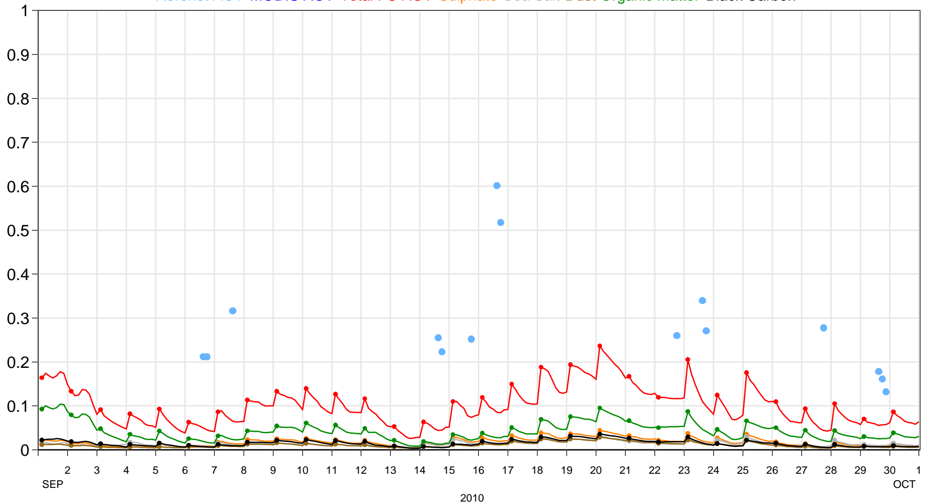
Comparison of model (f93i) and MODIS AOT at 550nm and L1.5 Aeronet AOT at 500nm over Arica (18.47° S, 70.31° W). Model: 00UT, 1-30 Sep 2010, T+3 to T+24.
