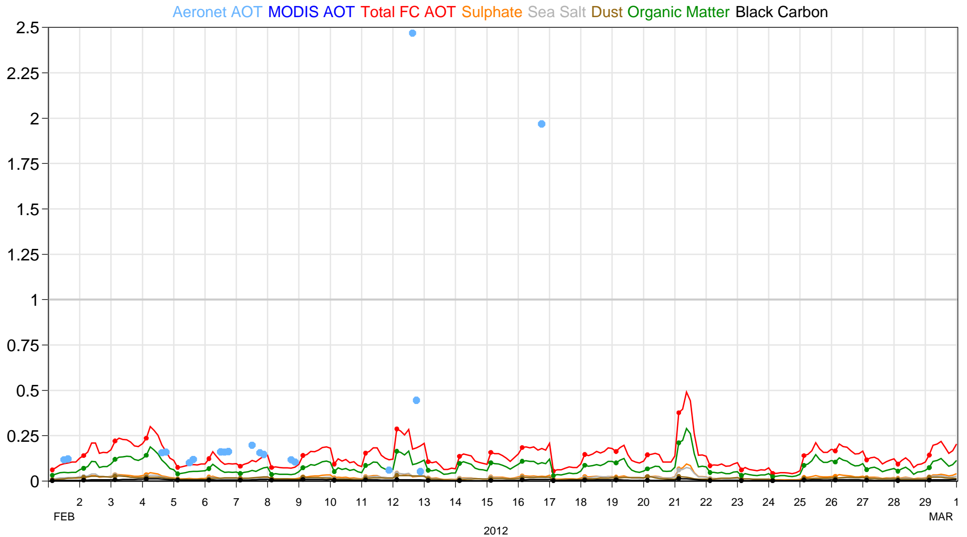
Comparison of model (fh9z) and MODIS AOT at 550nm and L1.5 Aeronet AOT at 500nm over Alta_Floresta (9.87° S, 56.1° W). Model: 00UT, 1-29 Feb 2012, T+3 to T+24.
