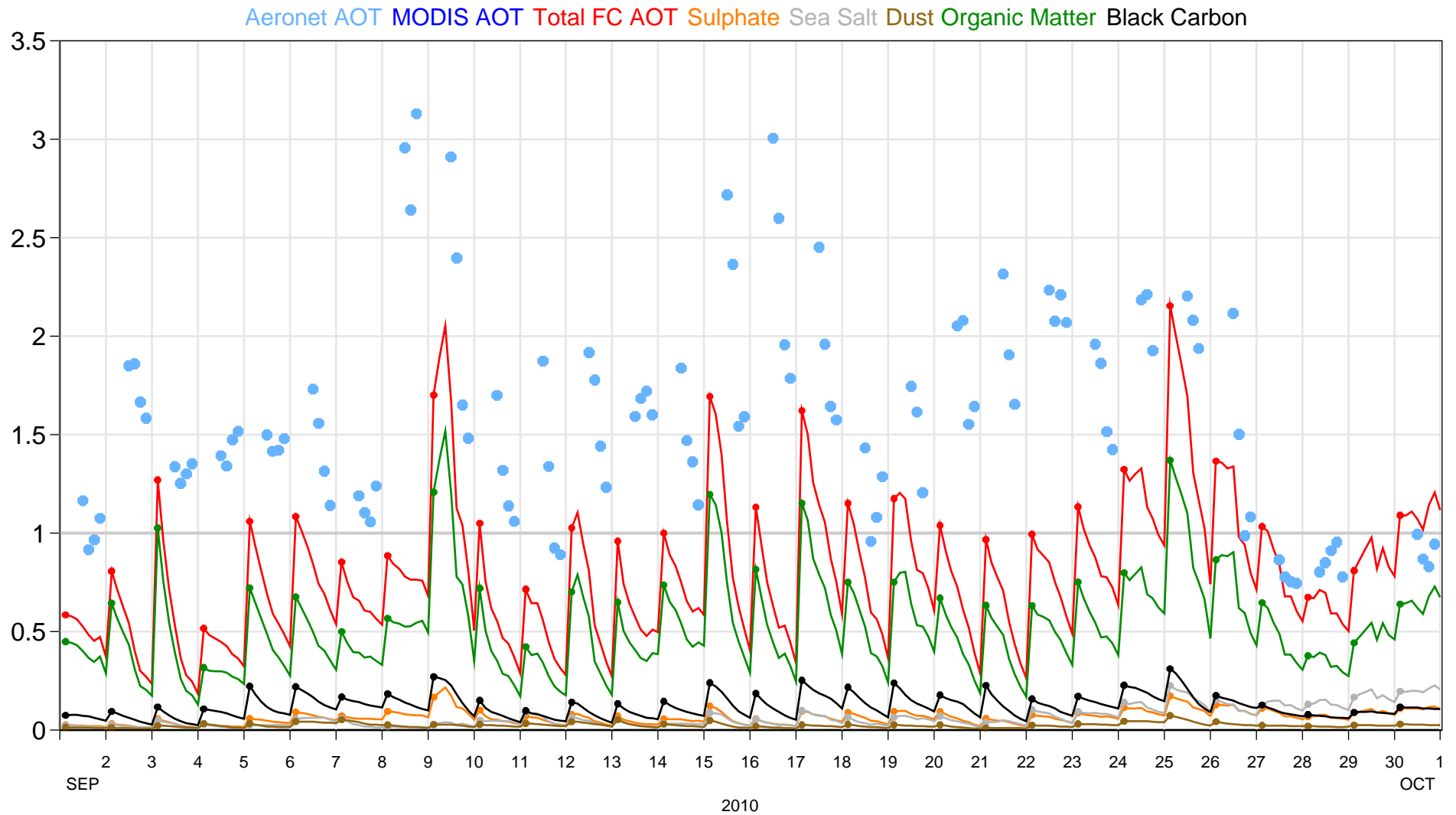
Comparison of model (f93i) and MODIS AOT at 550nm and L1.5 Aeronet AOT at 500nm over Alta_Floresta (9.87° S, 56.1° W). Model: 00UT, 1-30 Sep 2010, T+3 to T+24.
